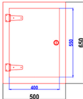
S1 GRP CABINET FRONT WALL ELEVATION WALL 1
