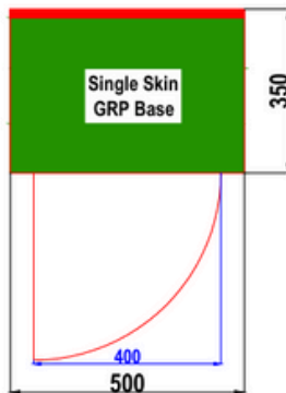
S1 GRP CABINET PLAN VIEW
