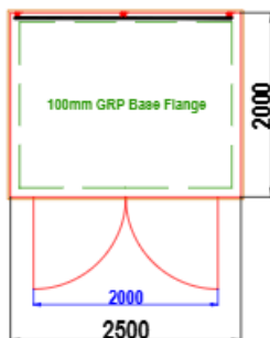
W5 WALK-IN GRP ENCLOSURE PLAN VIEW
