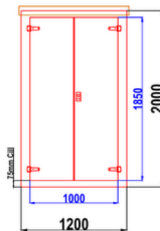
D6 GRP WALK-IN CABINET FRONT WALL ELEVATION WALL 1
