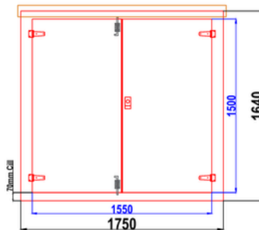
D4 GRP CABINET FRONT WALL ELEVATION WALL 1
