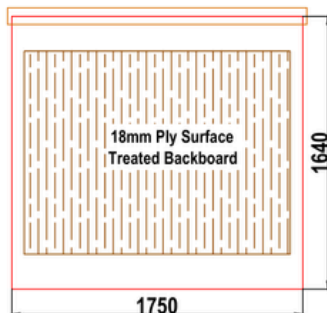
D4 GRP CABINET REAR WALL ELEVATION WALL 4
