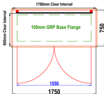
D4 GRP CABINET PLAN VIEW
