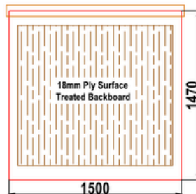
D2 GRP CABINET REAR WALL ELEVATION WALL 4
