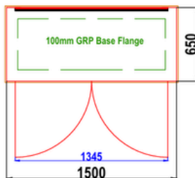
D2 GRP CABINET PLAN VIEW
