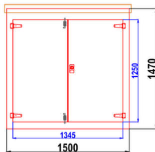
D2 GRP CABINET FRONT WALL ELEVATION WALL 1
