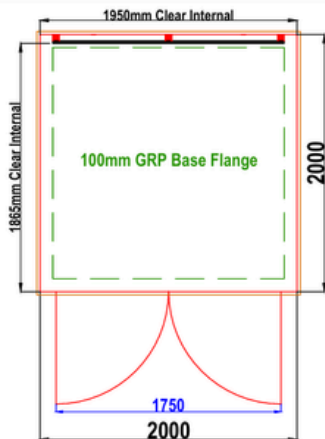
W4 GRP WALK-IN CABINET PLAN VIEW
