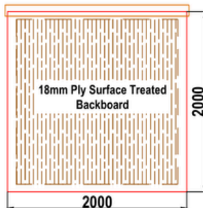
W4 GRP WALK-IN CABINET REAR WALL ELEVATION WALL 4
