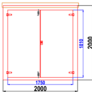
W4 GRP WALK-IN CABINET FRONT WALL ELEVATION WALL 1
