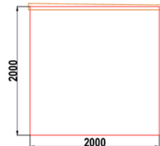
W4 GRP WALK-IN CABINET RIGHT HAND SIDE WALL ELEVATION WALL 3
