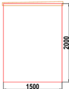
W3A GRP WALK-IN CABINET LEFT HAND SIDE WALL ELEVATION WALL 2
