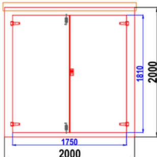
W3A GRP WALK-IN CABINET FRONT WALL ELEVATION WALL 1
