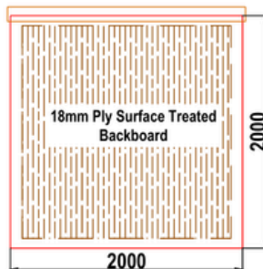
W3A GRP WALK-IN CABINET REAR WALL ELEVATION WALL 4
