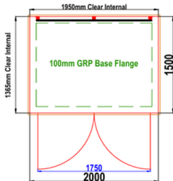
W3A GRP WALK-IN CABINET PLAN VIEW
