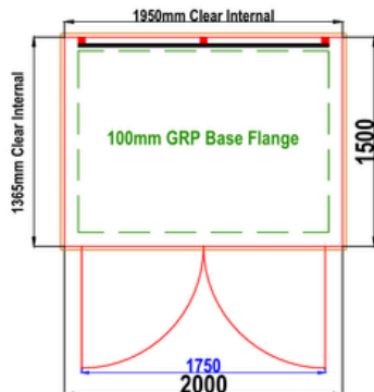
W3 GRP WALK-IN CABINET PLAN VIEW
