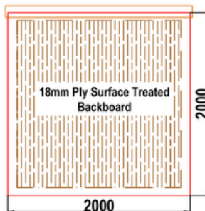
W3 GRP WALK-IN CABINET REAR WALL ELEVATION WALL 4
