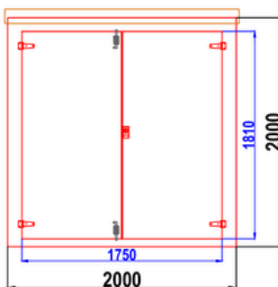
W2 GRP WALK-IN CABINET FRONT WALL ELEVATION WALL 1
