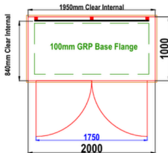
W2 GRP WALK-IN CABINET PLAN VIEW
