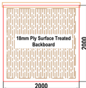
W2 GRP WALK-IN CABINET REAR WALL ELEVATION WALL 4
